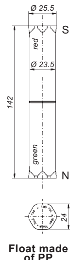
HA/PP with float made of PP and 2 magnetic switches
