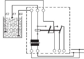
Circuit diagram: E0 = earth electrode, E1 and E2 = control electrodes
