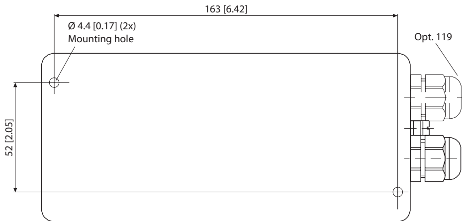
Rear view
